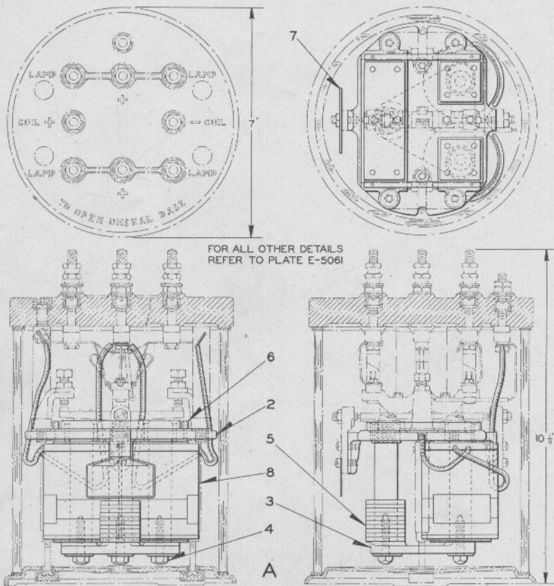
STYLE "NF-2" D. C. FLASHER RELAY
