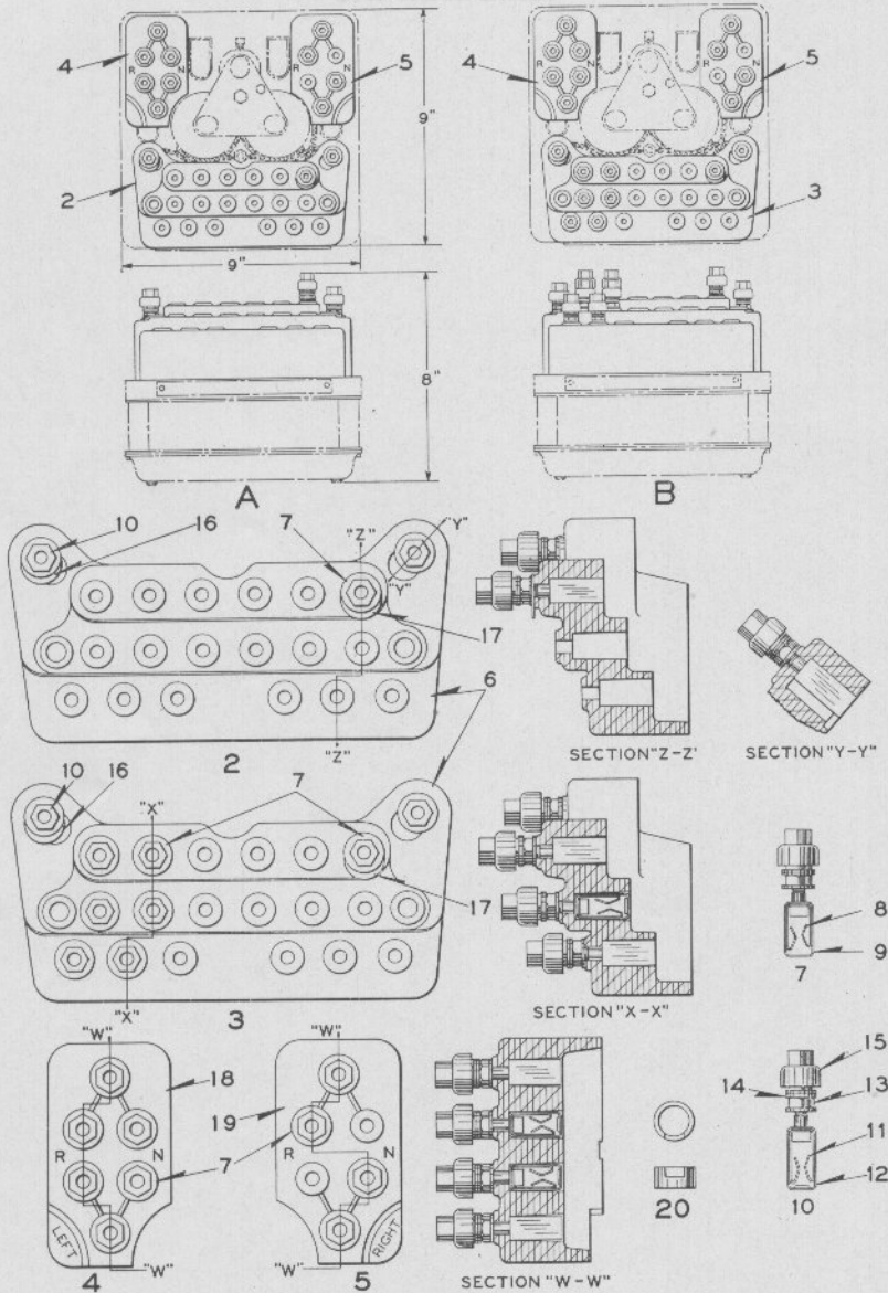
Plug Couplers for D. C. Relays ("DP-25" Having 4N-4R Polar Contacts)
