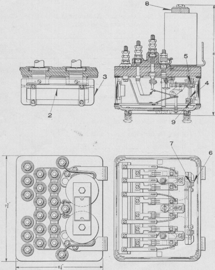
DETAILS OF "DN-12" D. C. TRUNNIONLESS NEUTRAL RELAY (SIX-POINT)
