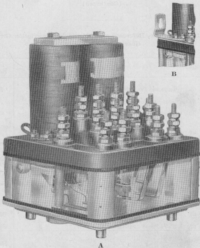
STYLE DN-11 D. C. NEUTRAL RELAY (FOUR-POINT)
