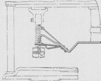
APPLICATION OF KNIFE EDGE BACK CONTACTS TO MODEL 13 TWO POINT ROUND BASE RELAY
