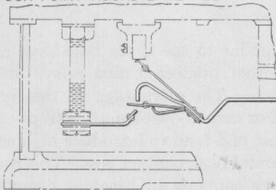
APPLICATION OF KNIFE EDGE BACK CONTACTS TO MODEL 13 SQUARE BASE RELAY.
