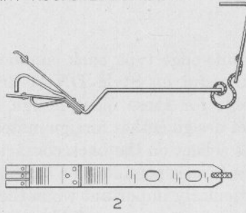
APPLICATION OF KNIFE EDGE BACK CONTACTS TO MODEL 13 TWO POINT ROUND BASE RELAY
