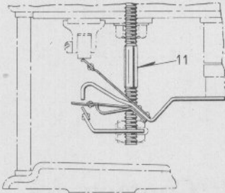
APPLICATION OF KNIFE EDGE BACK CONTACTS TO MODEL 13 FOUR POINT ROUND BASE RELAY
