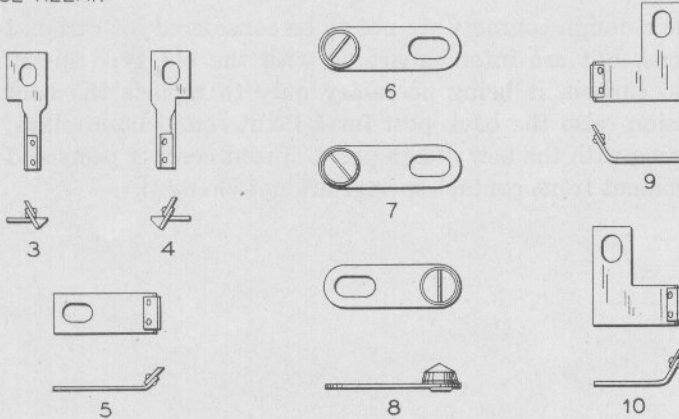
APPLICATION OF KNIFE EDGE BACK CONTACTS TO MODEL 13 SQUARE BASE RELAY.
