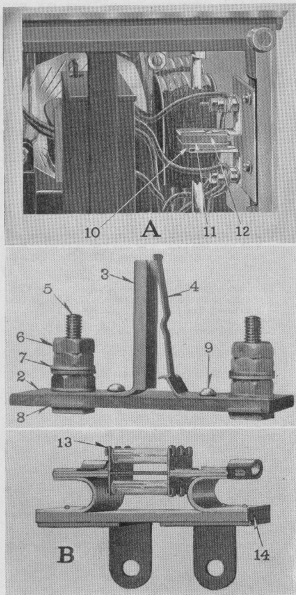
LIGHTNING ARRESTER FOR MODEL 15 AND SLV-13 VANE RELAYS
