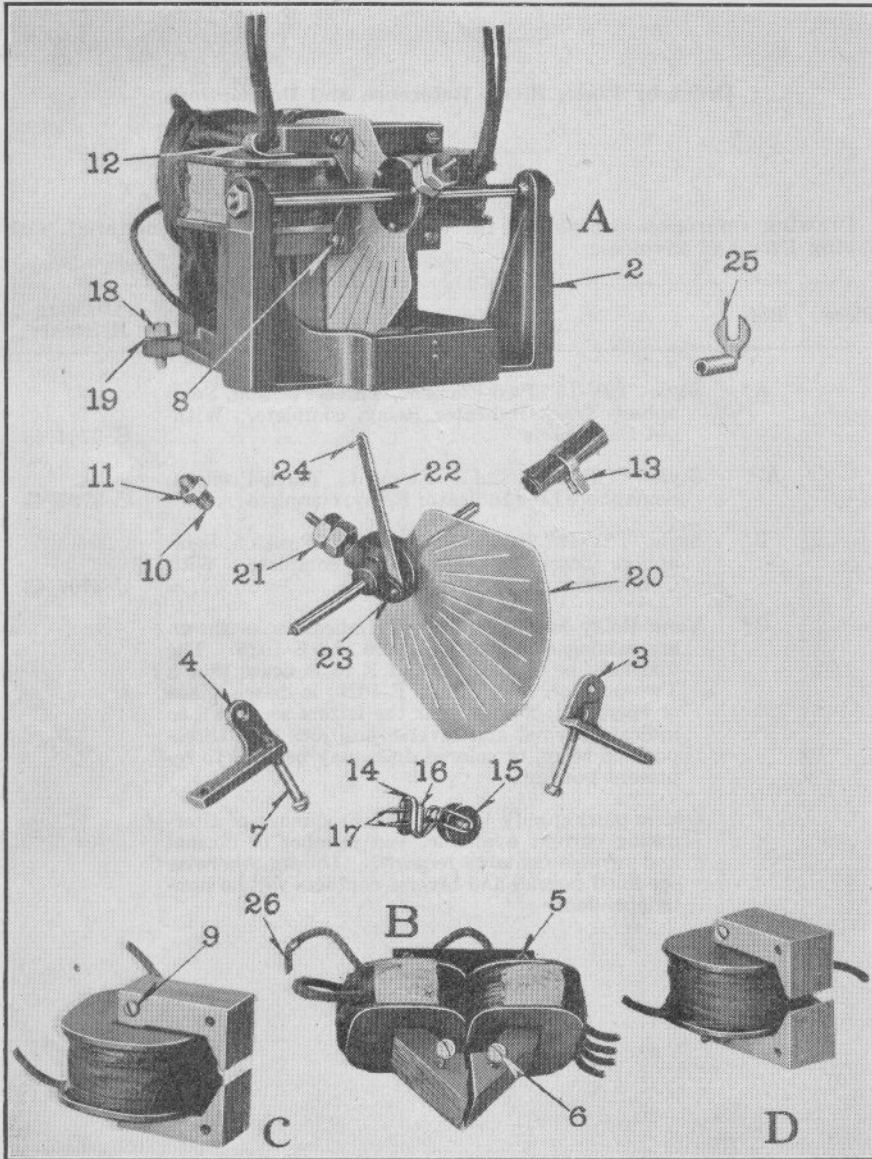
OPERATING MECHANISM AND DETAILS FOR TWO AND THREE POSITION MODEL 15 VANE RELAY
