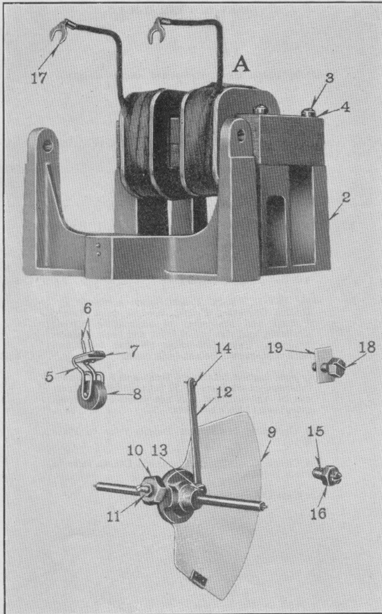
OPERATING MECHANISM AND DETAILS FOR SV-12 VANE RELAY
