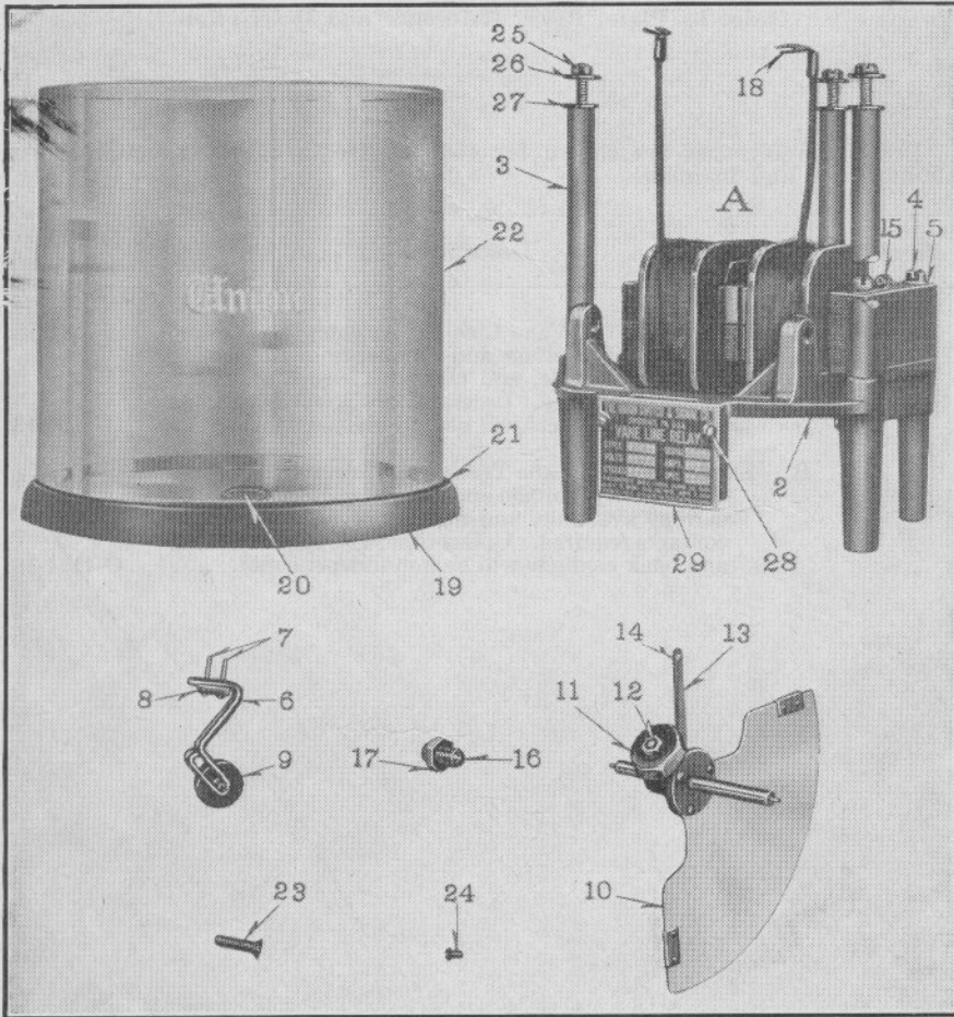
OPERATING MECHANISM AND DETAILS FOR SLV-13 VANE RELAY
