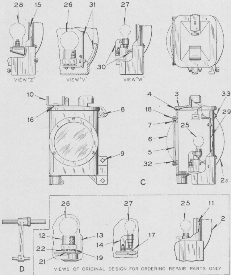
Style "D" Cast Iron Semaphore Lamp And Sighting Tube
