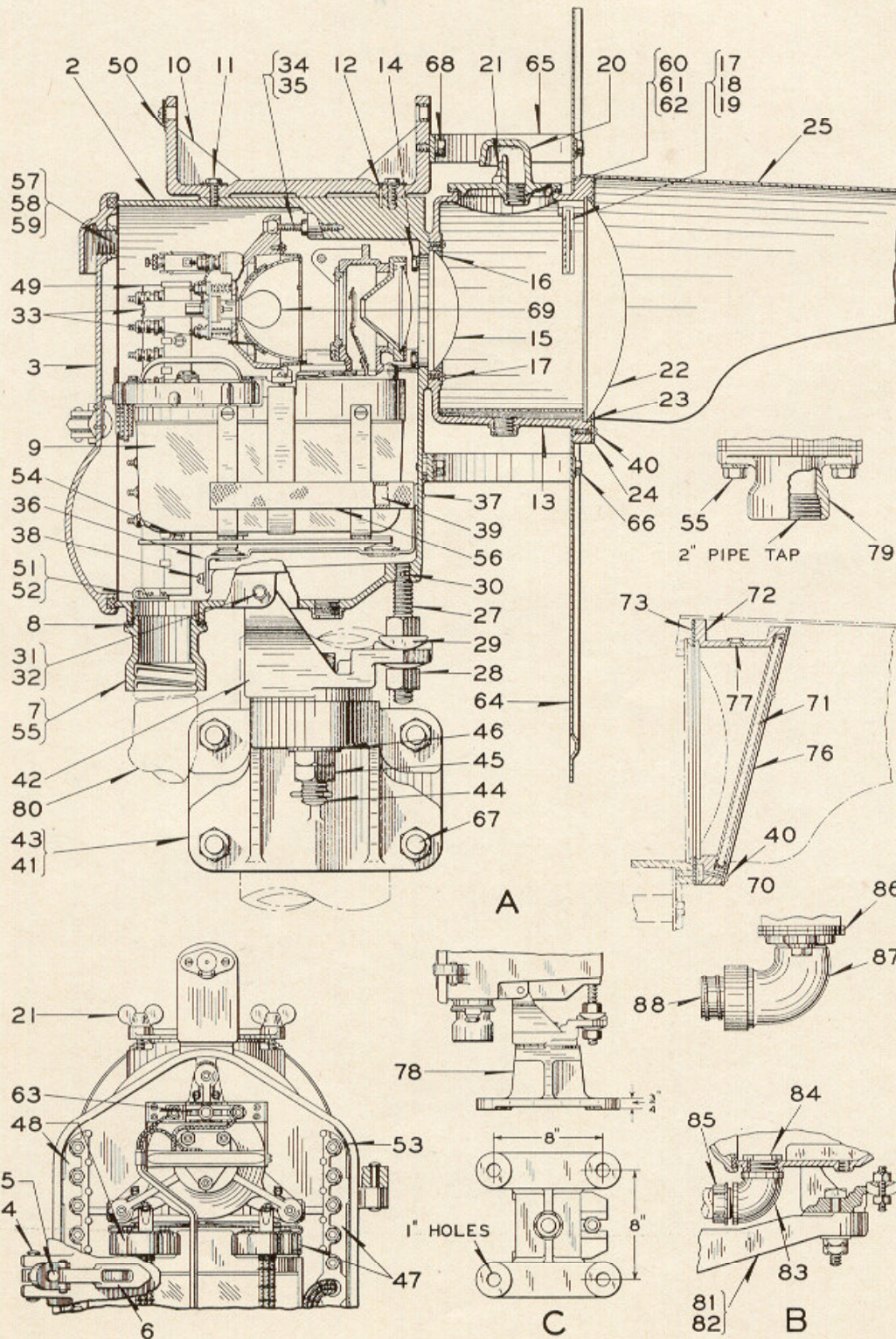
Style "H-5" Searchlight Signal Unit
