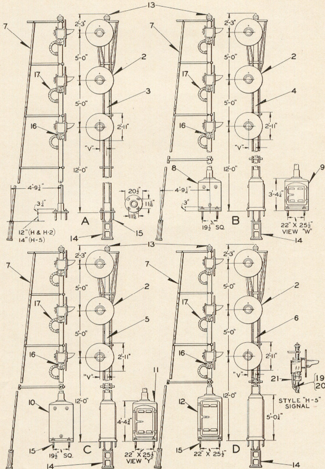
Three Unit, Styles "H", "H-2" and "H-5" Searchlight Ground Signals
