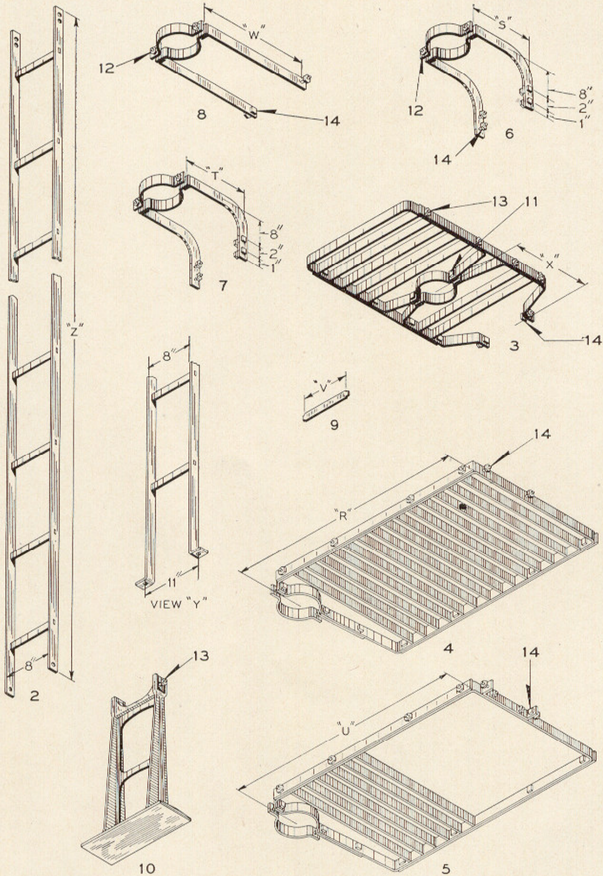
Ladder Details for Color Light Signals
