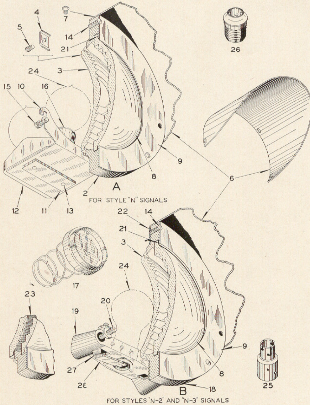
Lamp Unit Assemblies for Styles "N", "N-2", "N-3", "TN" and "TN-2" Light Signal Units
