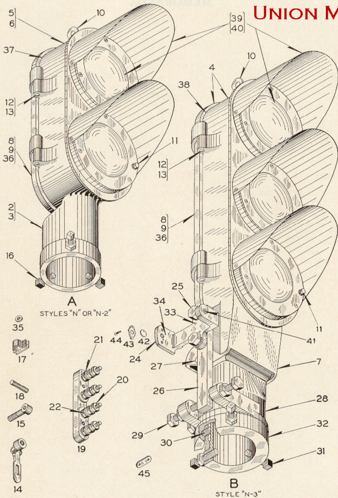
Two and Three-Color Styles "N", "N-2" and "N-3" Signal Units (Without Backgrounds)
