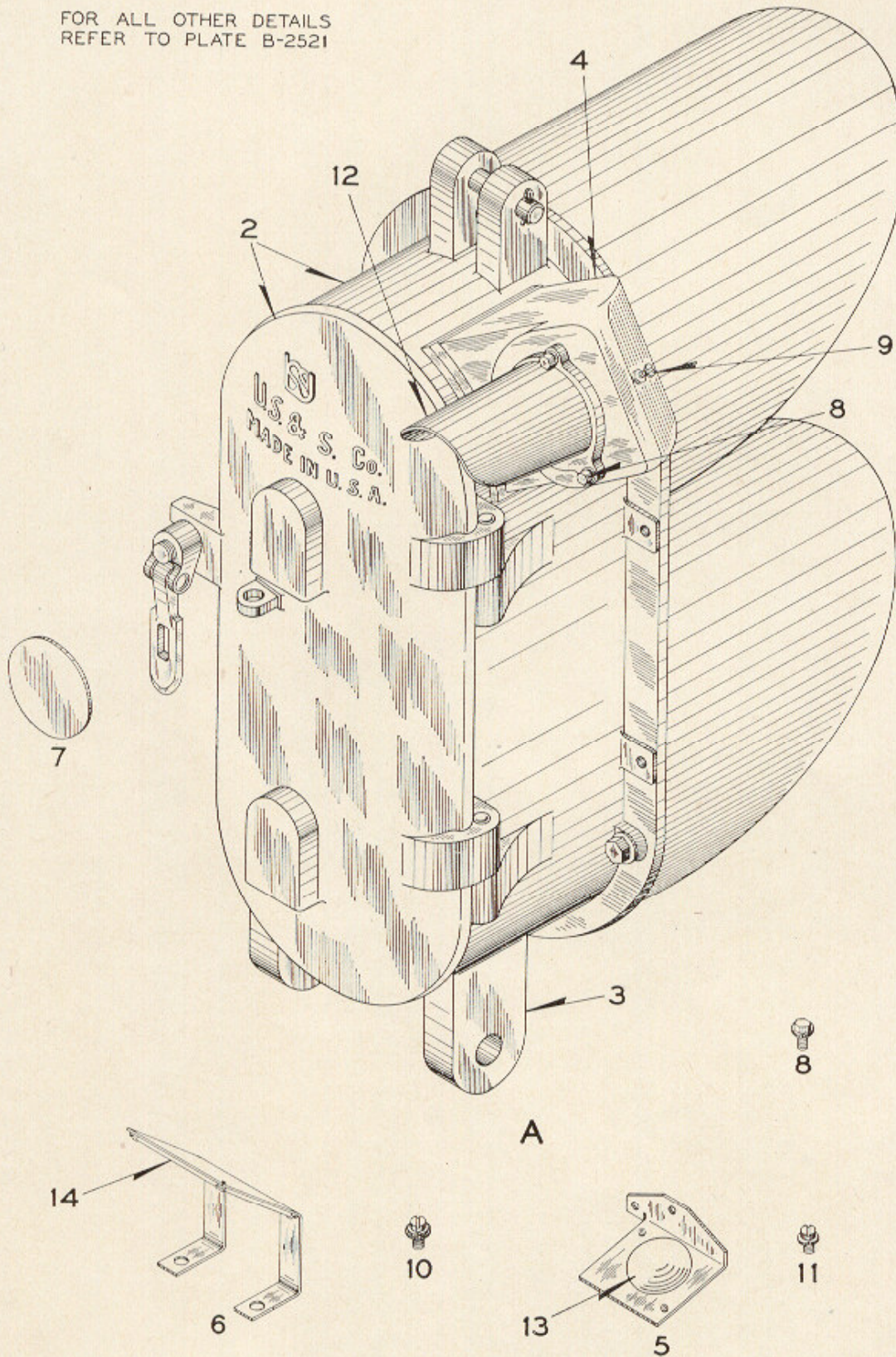
Two and Three-Color Style "R-2" Signal Units with Backlight on Top Lamp Unit (Without Backgrounds)
