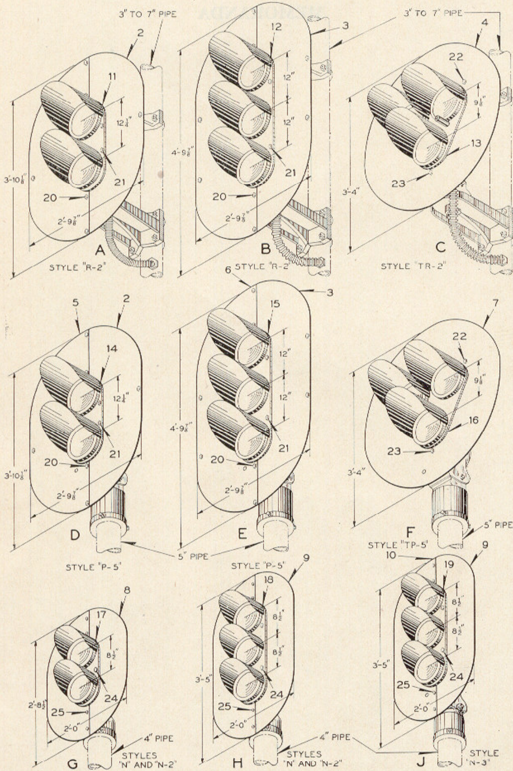
Two and Three-Color Styles "R-2", "P-5", "N", "N-2", "N-3", "TR-2" and "TP-5" Signal Units
