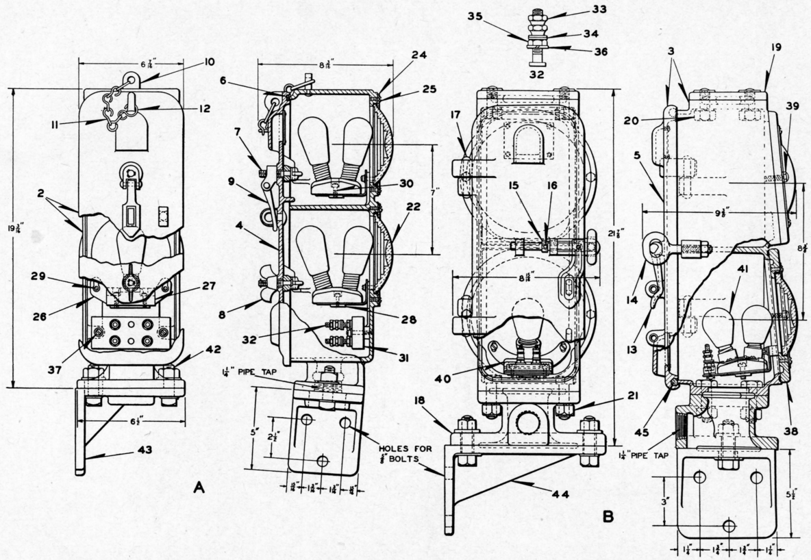
TWO-COLOR SUBWAY LIGHT DWARF SIGNAL WITH BRACKET MOUNTING
