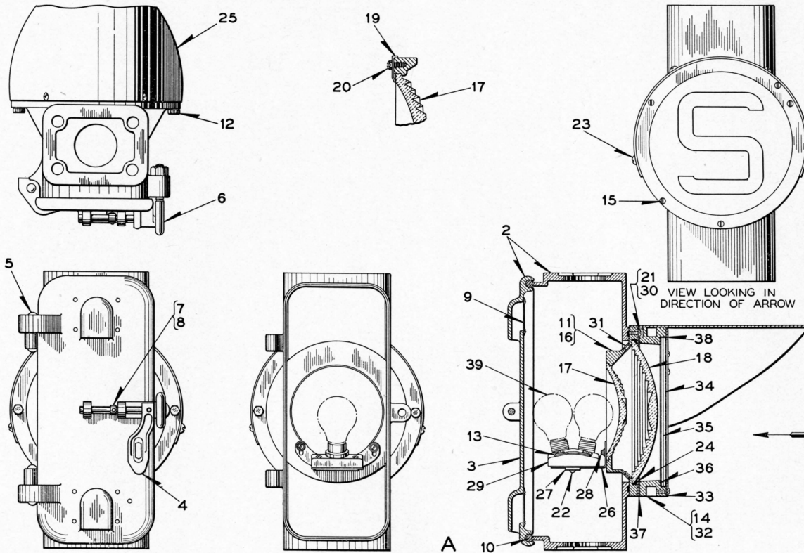
ONE-COLOR LIGHT SIGNAL UNIT WITH ILLUMINATED LETTER
