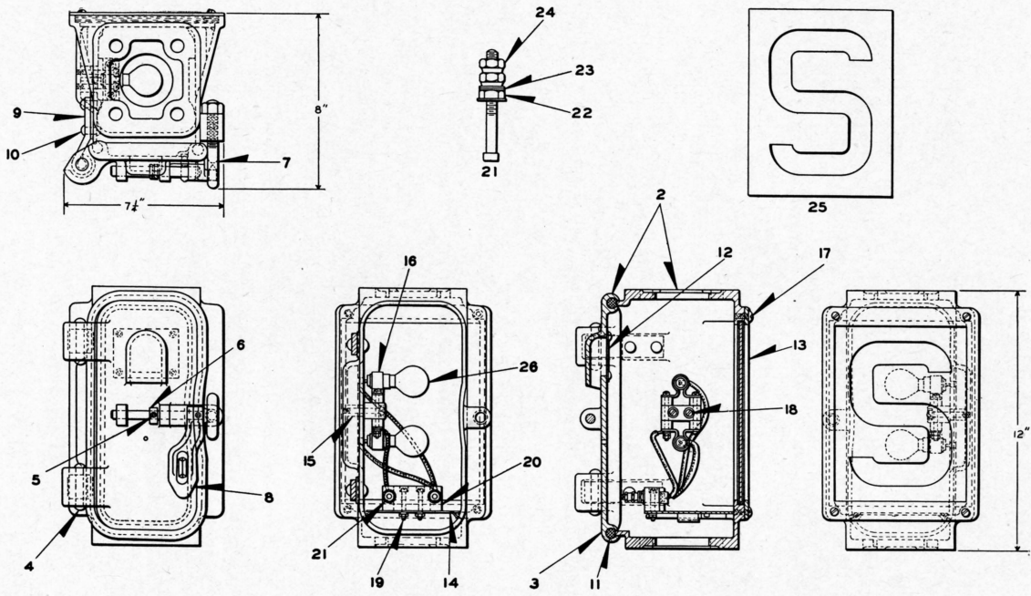
ILLUMINATED LETTER "S" UNIT FOR SUBWAY SIGNALS
