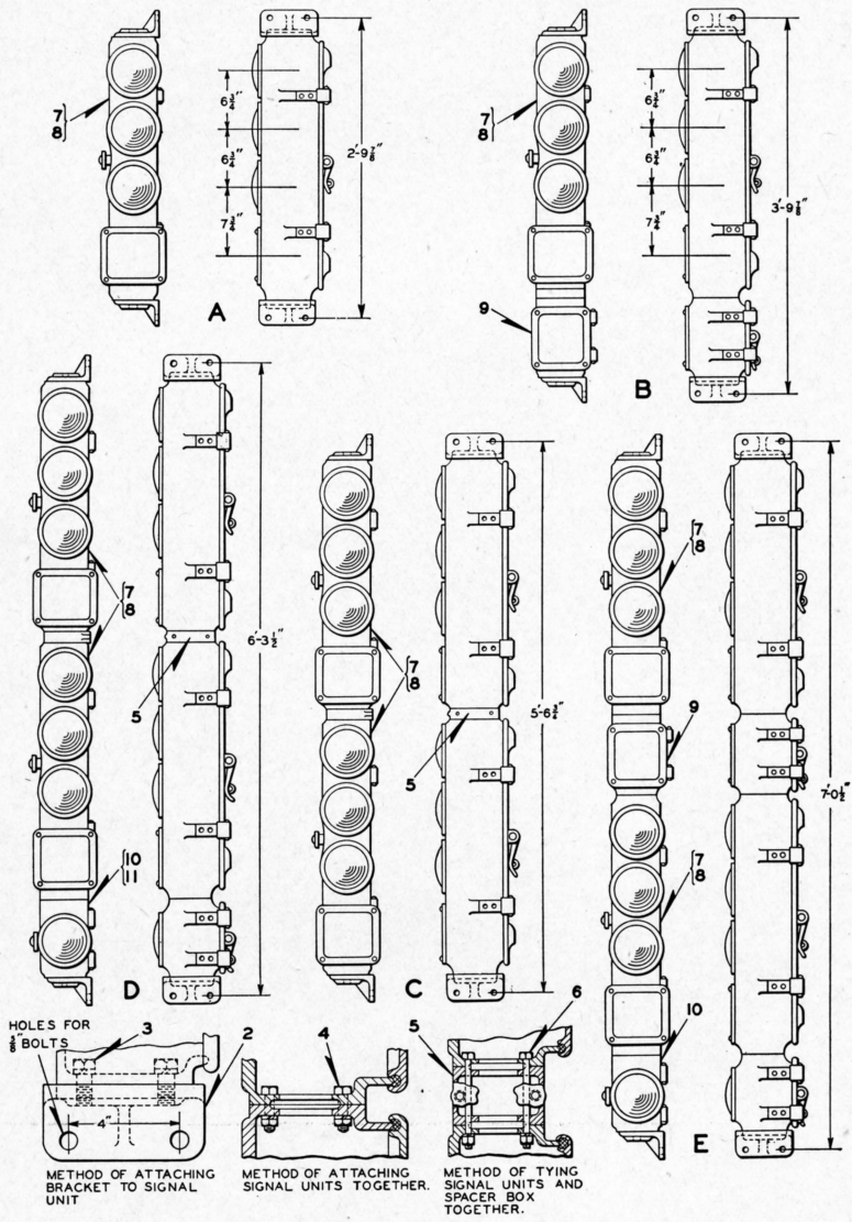
SUBWAY COLOR LIGHT SIGNALS WITH SINGLE 5" LENSES (MULTIPLE UNIT TYPE)
