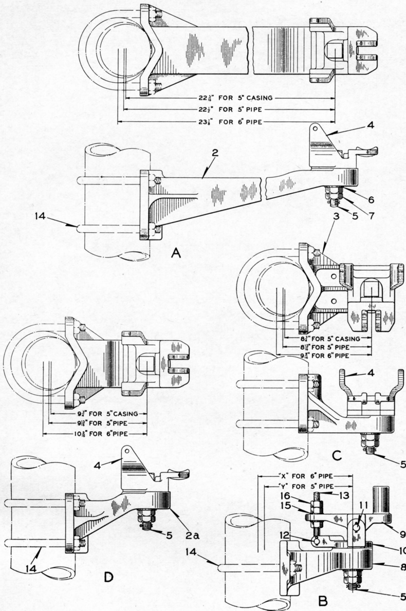
Mounting Brackets for Searchlight Signals and Marker Lights
