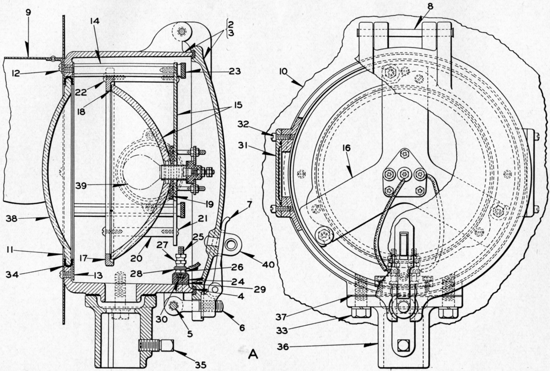
STYLE "HC-41" MARKER LIGHT UNIT
