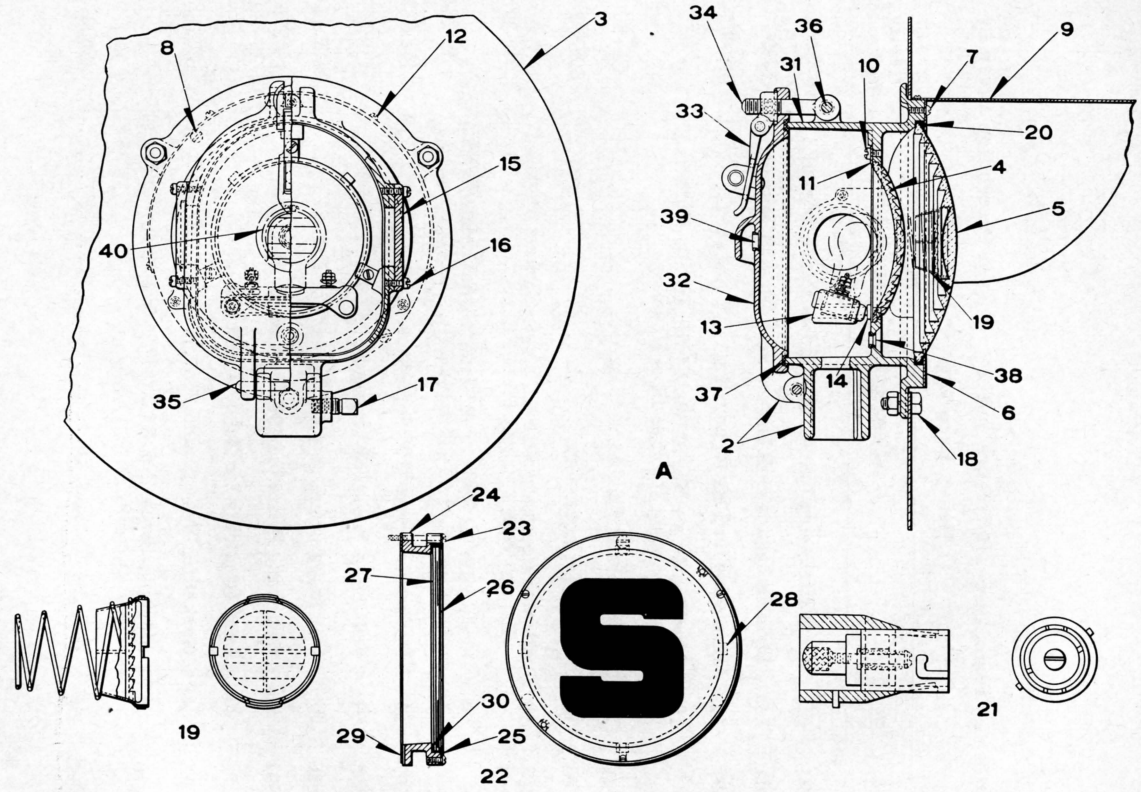
ONE-COLOR STYLE "R-2" LIGHT SIGNAL UNIT
