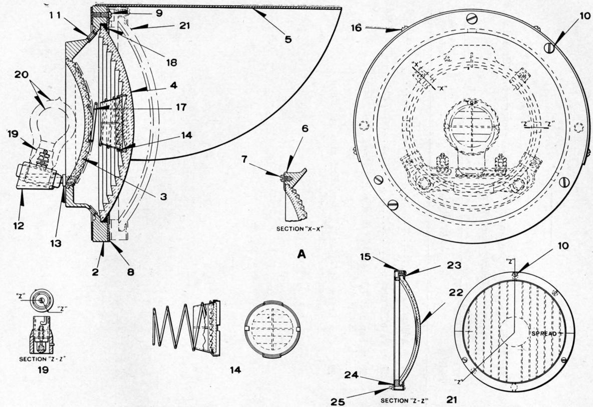
LAMP UNIT ASSEMBLY FOR STYLE "P-2" AND "TP-2" LIGHT SIGNAL UNITS
