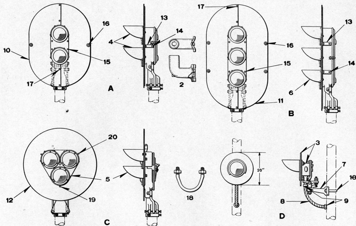
TWO AND THREE-COLOR STYLE "P-2" AND "TP-2" SIGNAL UNITS AND ONE-COLOR STYLE "R-2" SIGNAL UNIT
