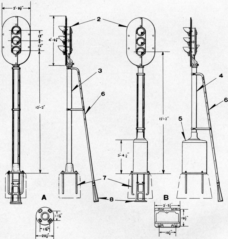
1-UNIT, THREE-COLOR STYLE "P-2" LIGHT GROUND SIGNALS
