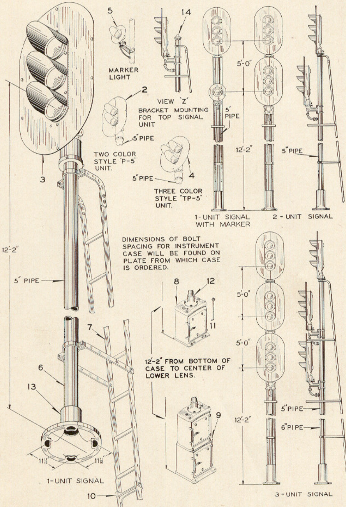
Styles "P-5" and "TP-5" Color Light Ground Signals
