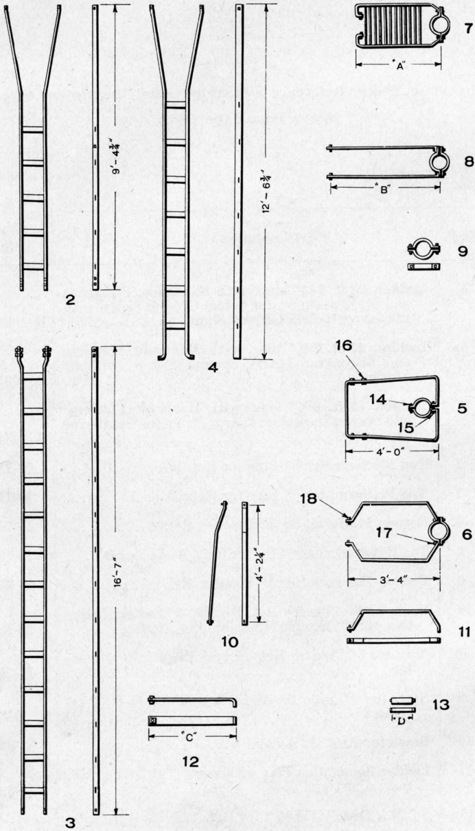
DETAILS OF LADDERS FOR POSITION LIGHT SIGNALS
