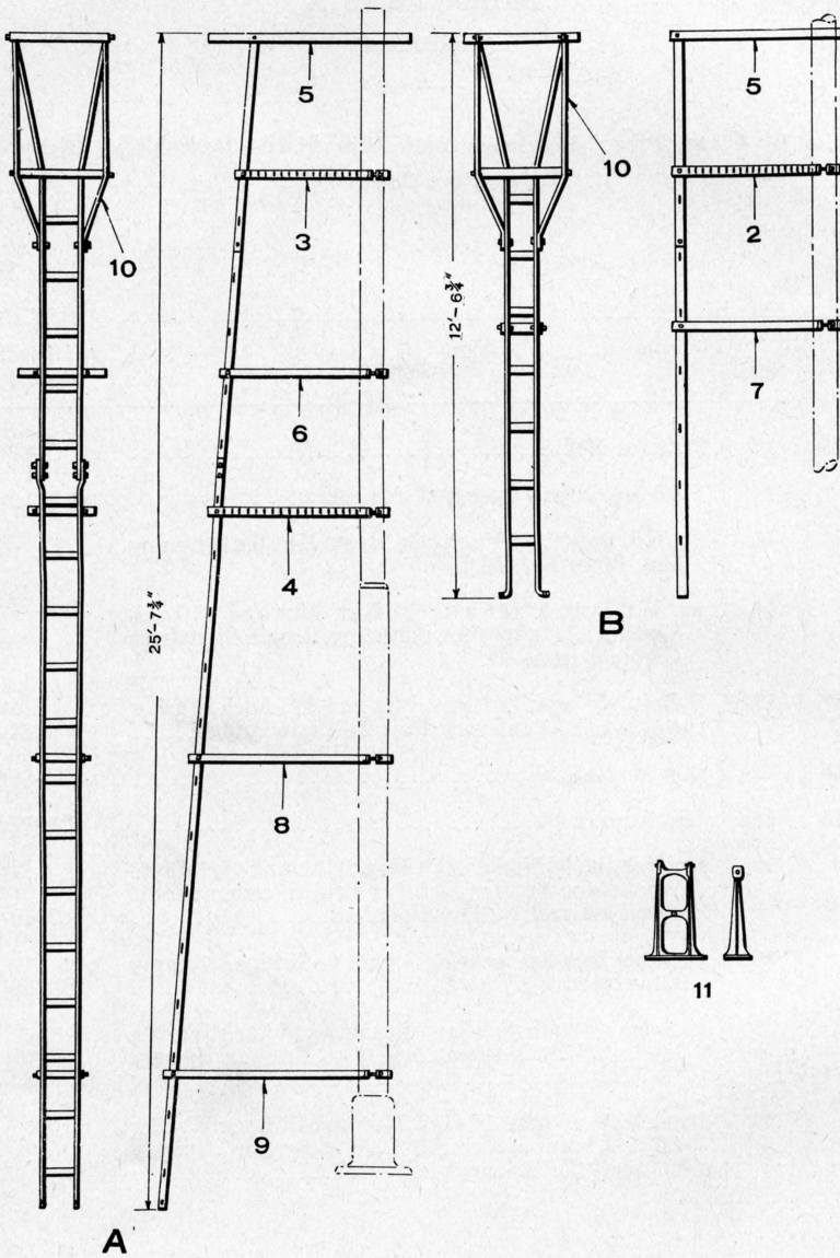
LADDERS FOR POSITION LIGHT SIGNAL
