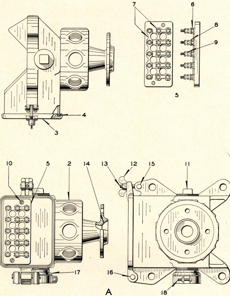
Combined Lamp Support and Terminal Box for Position Light Signals
