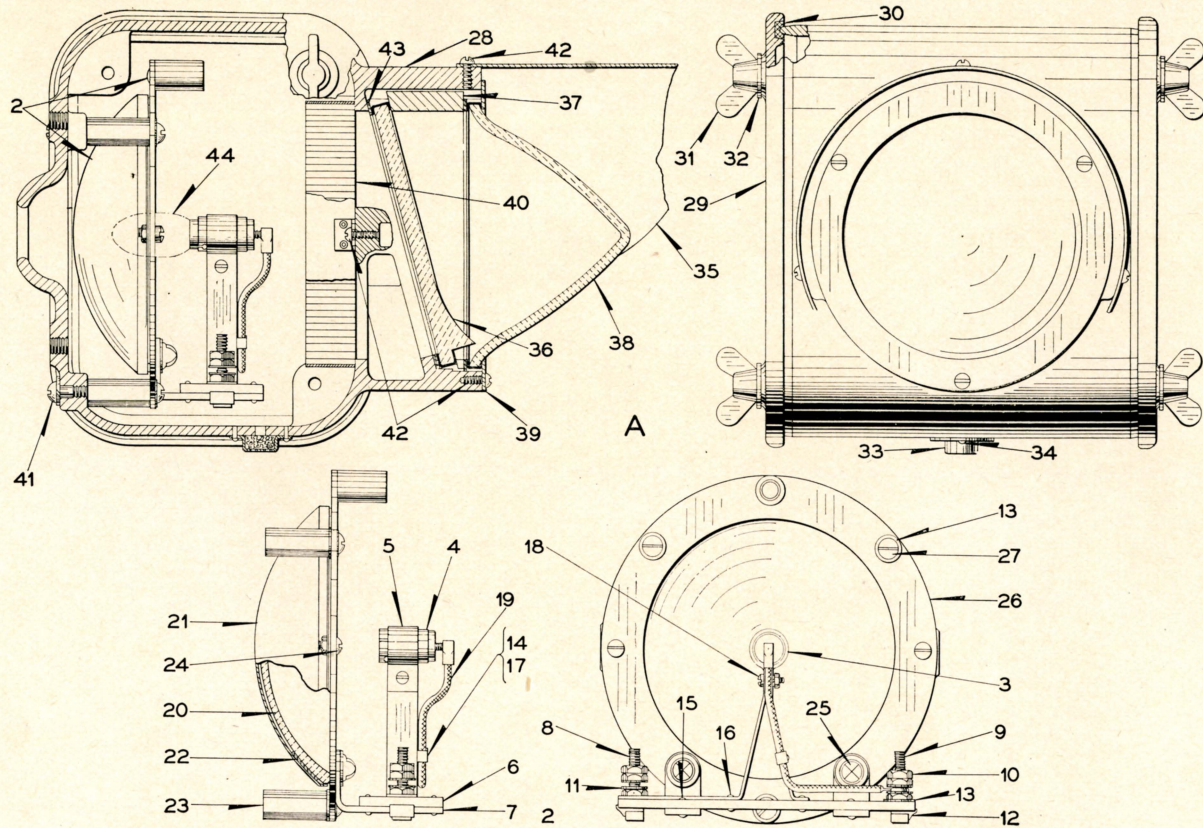
Lamp Unit for Style "PL-3" Position Light Signal
