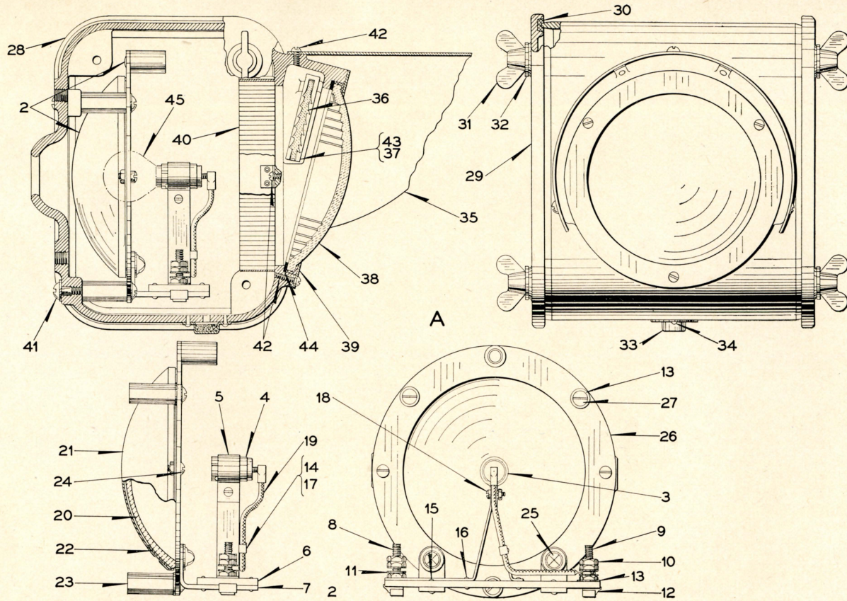
Lamp Unit for Style "PL-2" Position Light Signal
