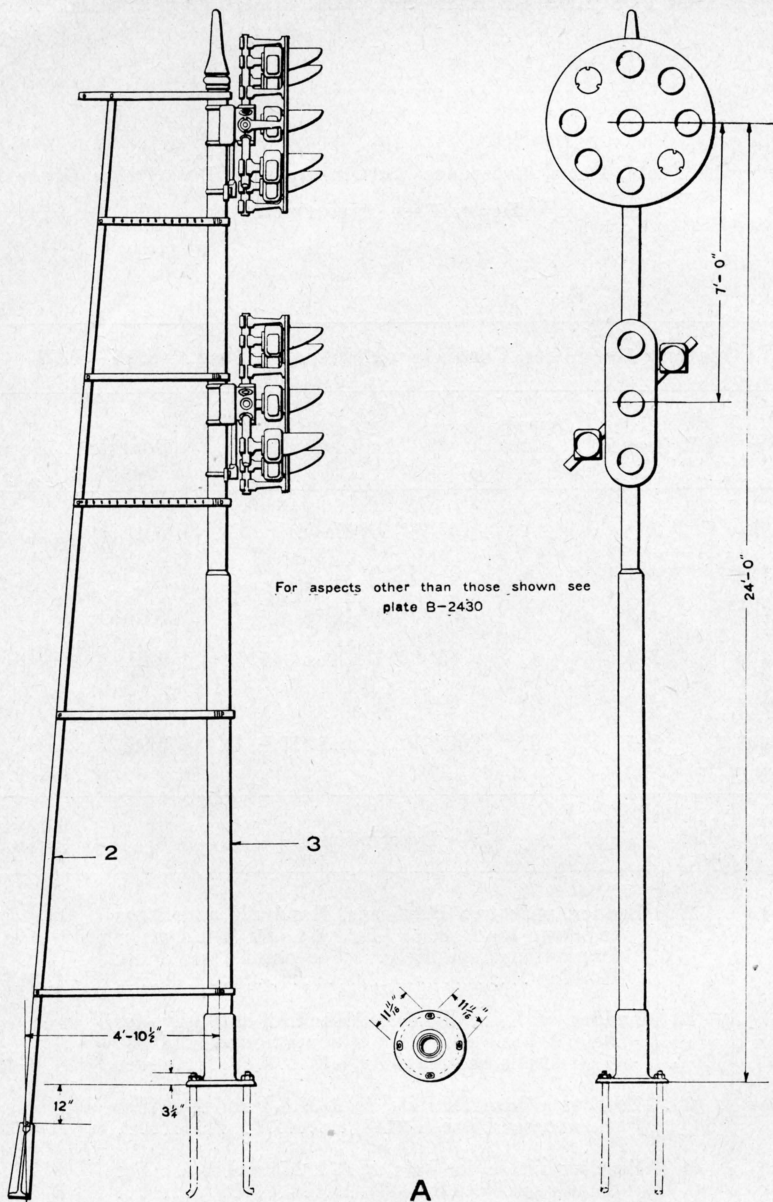
TWO ARM POSITION LIGHT GROUND SIGNAL
