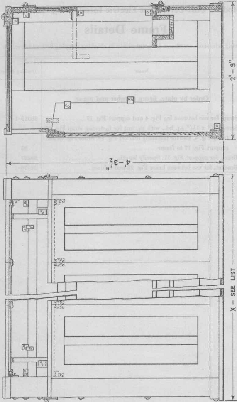
Cabinets for Model 2 Unit-Lever Type Electric Interlocking Machines
