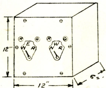
Sheet Steel Control Box Per Plan O-1233A
