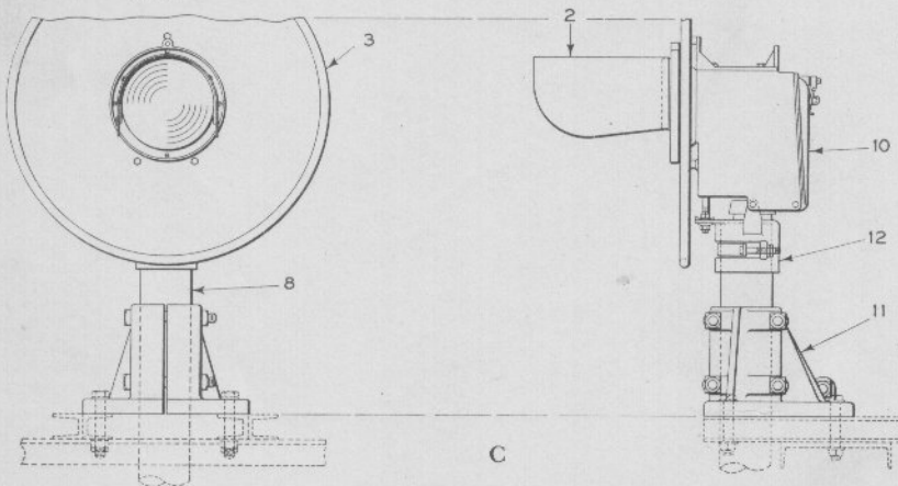
Type SA Color-Light Bridge Signals
