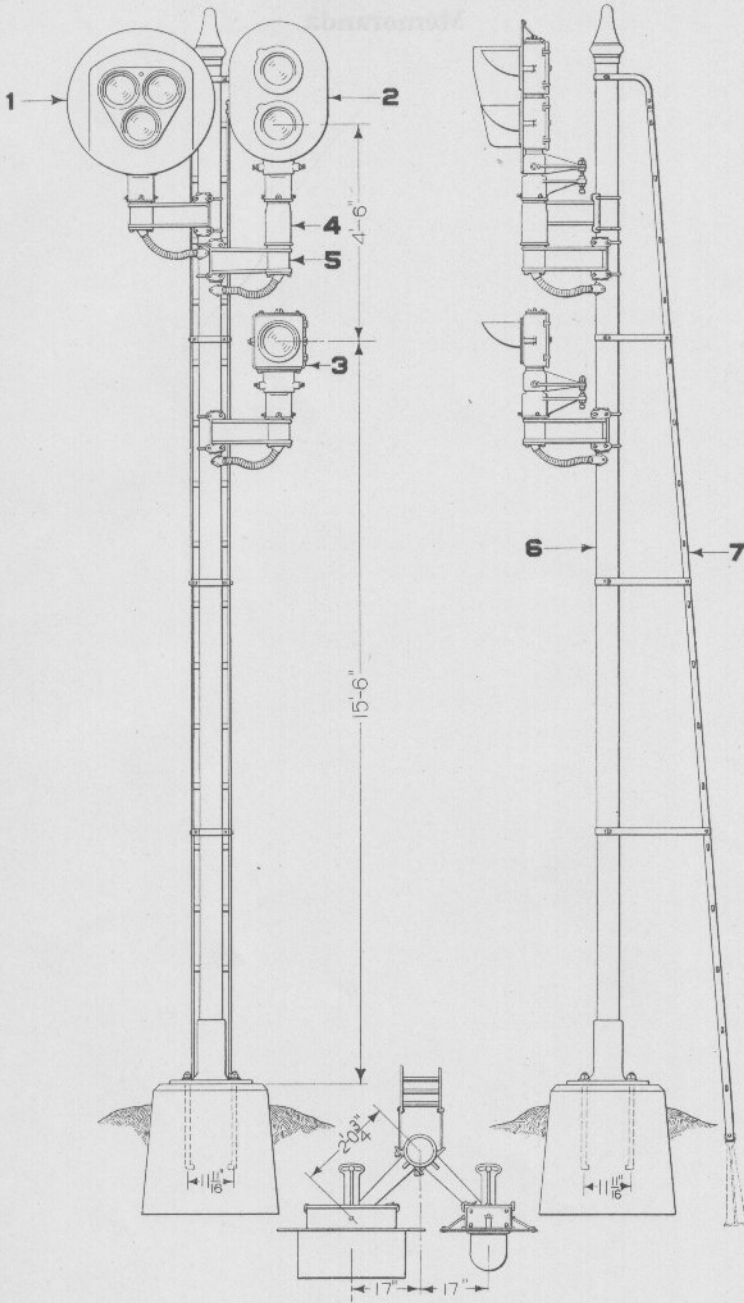
Combination Automatic and Train Order Signal
