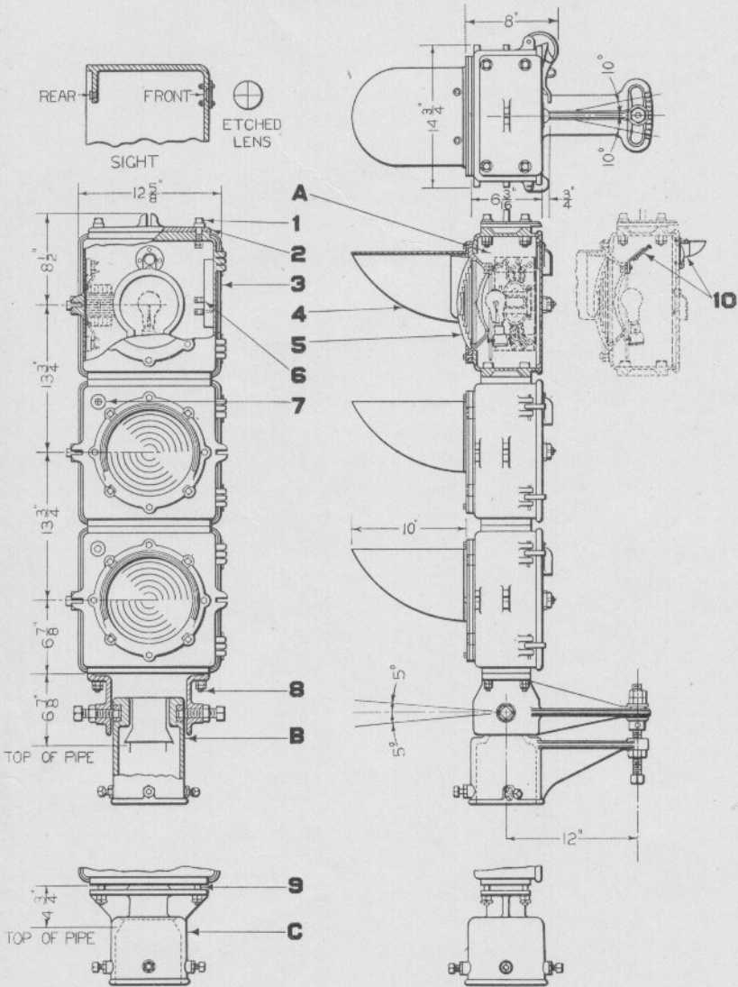
Type D Three Indication Light Signal Unit
