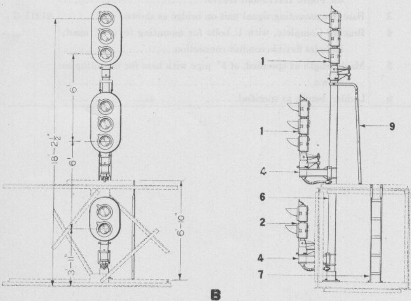
Type D Color Light Bridge Signals, Interlocking
