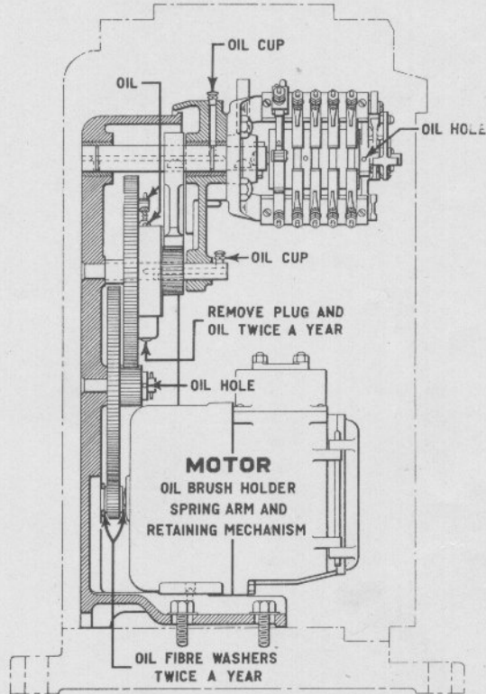
Model 2A Base-of-Mast Signal Mechanism
