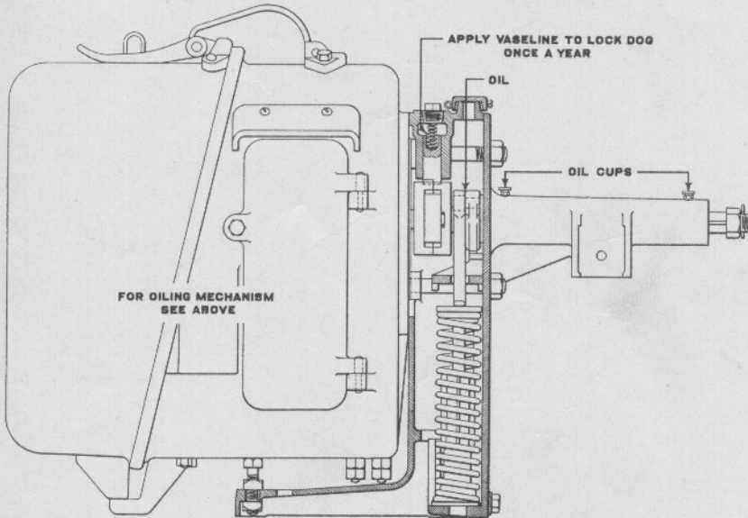
Model 2A Dwarf Signal
