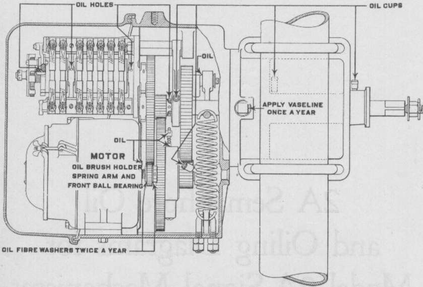
Model 2A Top-of-Mast Signal Mechanism
