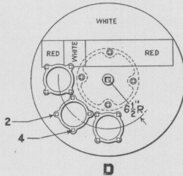
Disc Spectacles for Dwarf Signals
