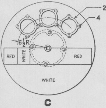
Disc Spectacles for Dwarf Signals
