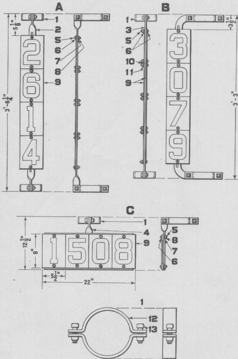
Number Plates for Mounting on Signal Masts
