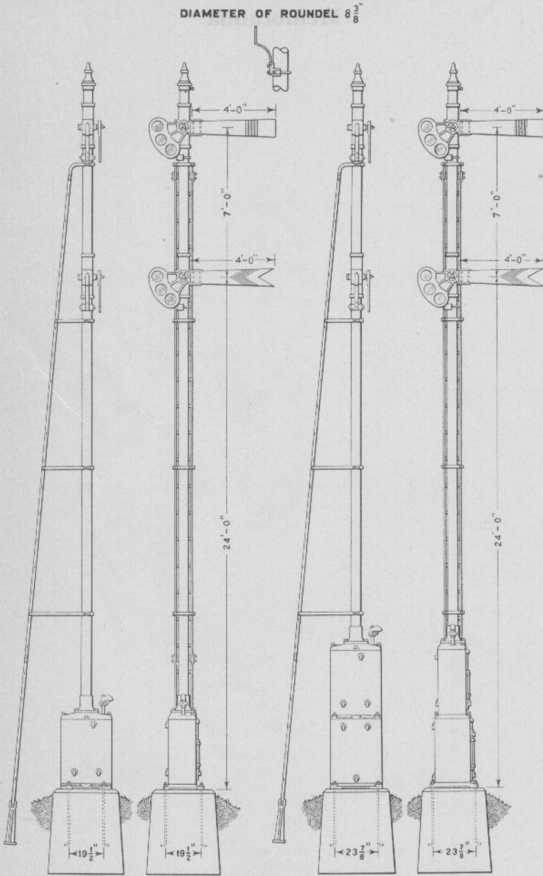
Two Arm Lower Quadrant Ground Signals Base of Mast Mechanism
