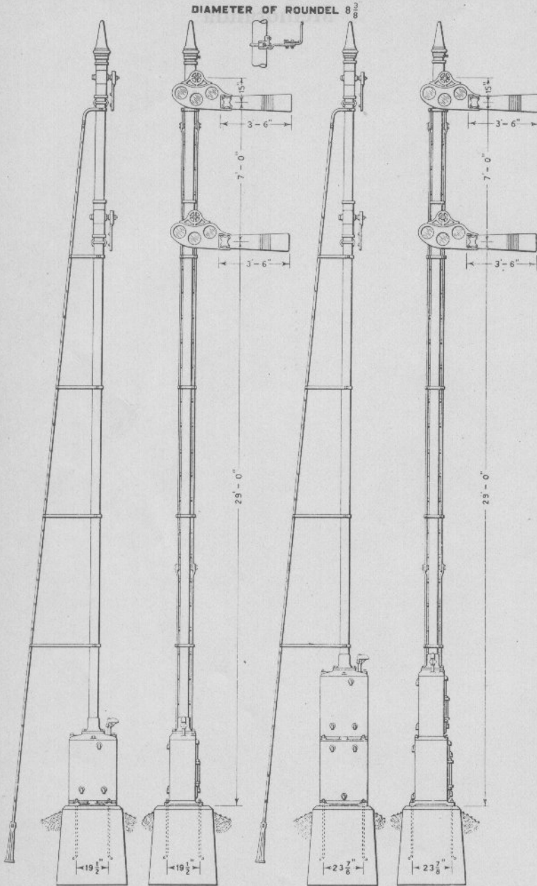
High Two Arm Upper Quadrant Ground Signals Base of Mast Mechanism
