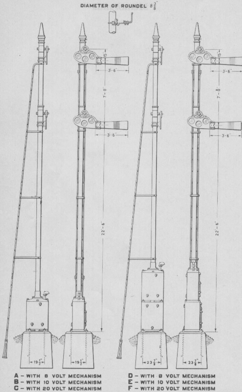
Two Arm Upper Quadrant Ground Signals Base of Mast Mechanism
