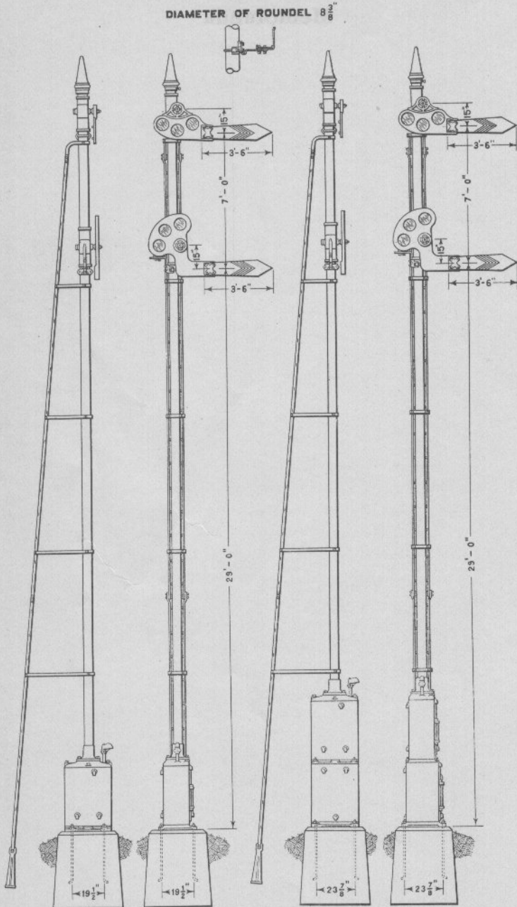
High Two Arm Upper Quadrant Ground Signals Base of Mast Mechanism
