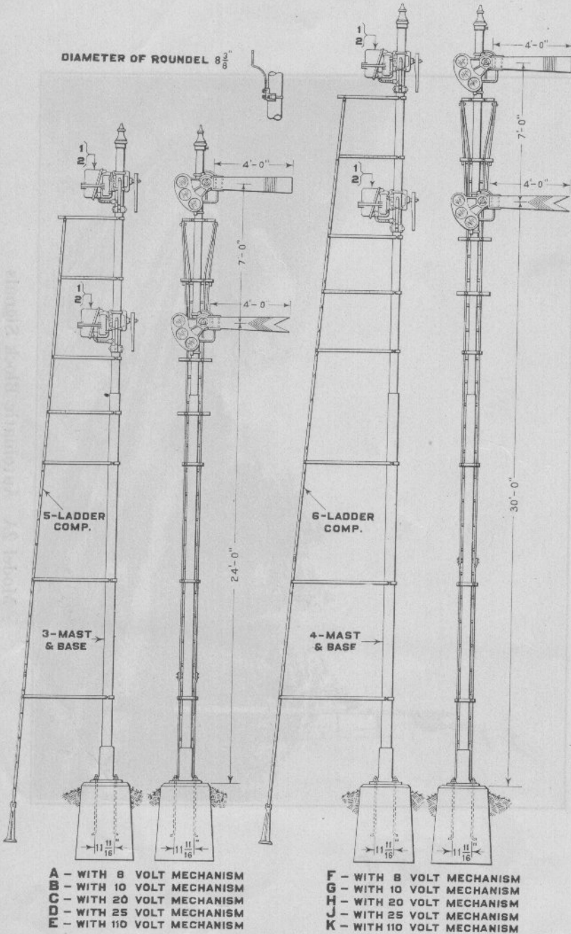
Two Arm Lower Quadrant Ground Signals
