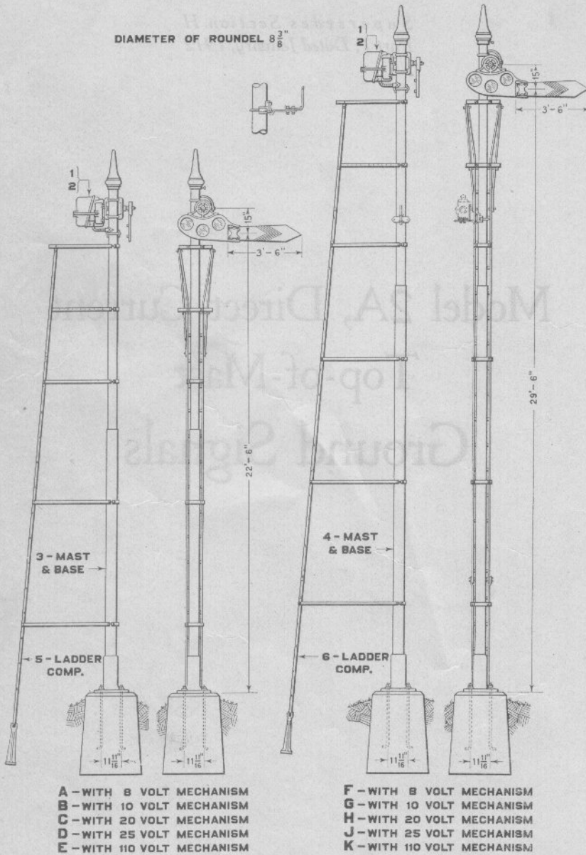
One Arm Upper Quadrant Ground Signals
