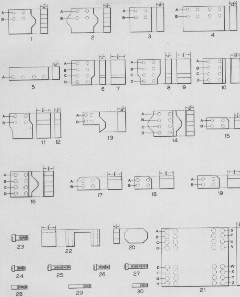
Locking Dogs and Guides For Interlocking Machines Modified Locking
